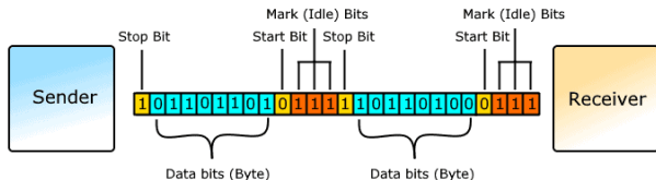
Asynchronous Transmission
